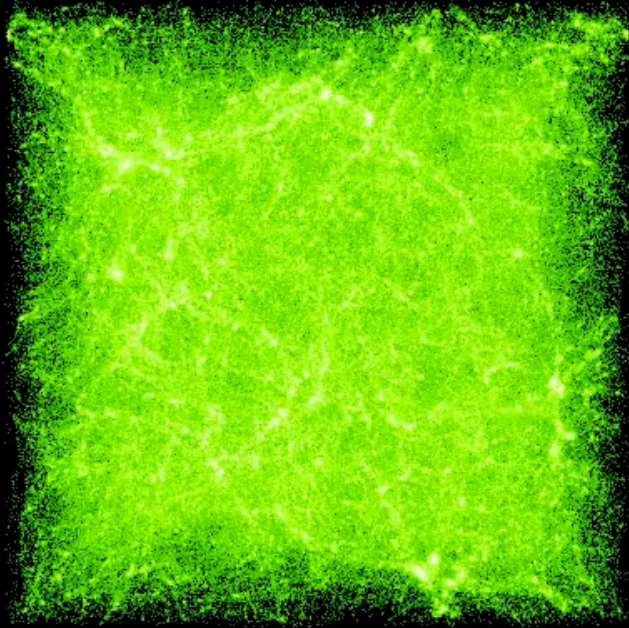
Lambda-CDM
