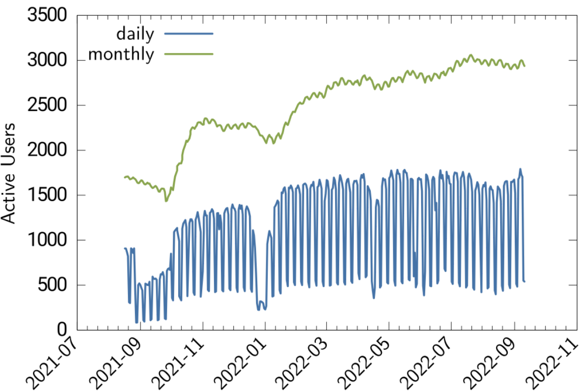
Mattermost
