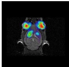
micro-PET
