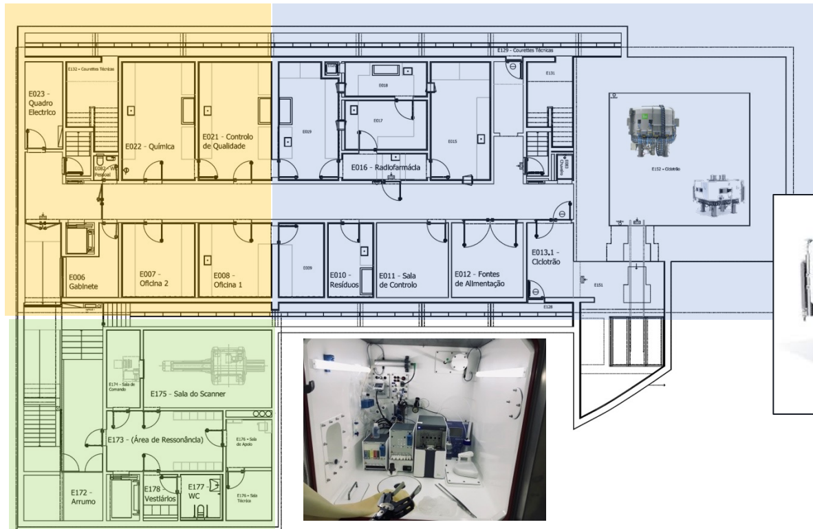
micro-PET
